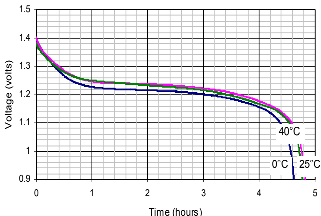
C/4 Discharge Profiles @ 0°C, 25°C, & 40°C
