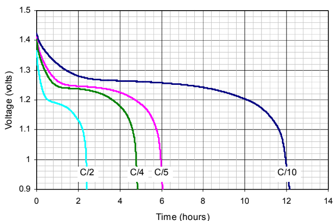
C/10-C/2 Discharge Profile @ 25°C
