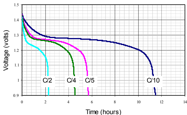
C/10-C/2 Discharge Profile @ 25°C
