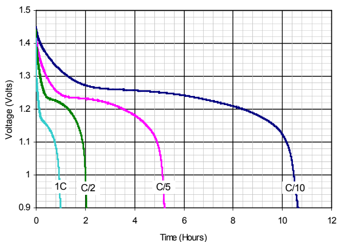
C/10-C Discharge Profile @ 25°C
