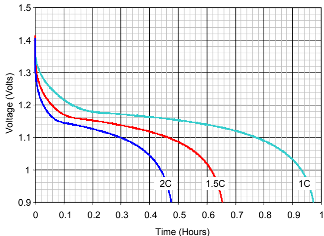
C-2C Discharge Profile
