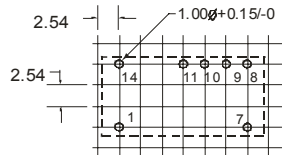
DXXXXXD-2W Footprint
