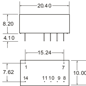
DXXXXXD-2W Package
