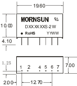
DXXXXXS-2W Footprint
