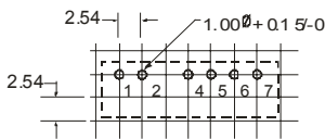
DXXXXXS-2W Footprint
