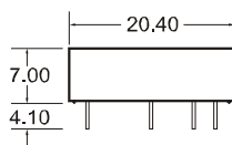
BXXXXLD-1W Package
