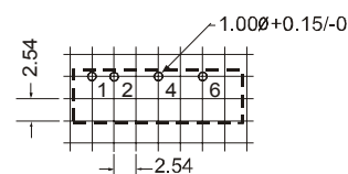
BXXXXLS-1W Package
