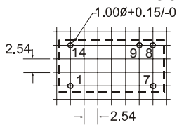
BXXXXLD-1W Package
