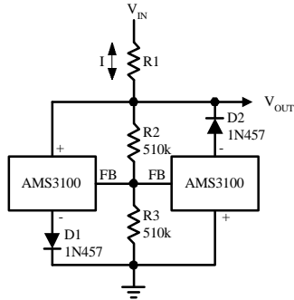
Bidirectional Clamp ± 2.4V
