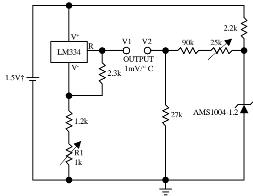
Centigrade Thermometer
